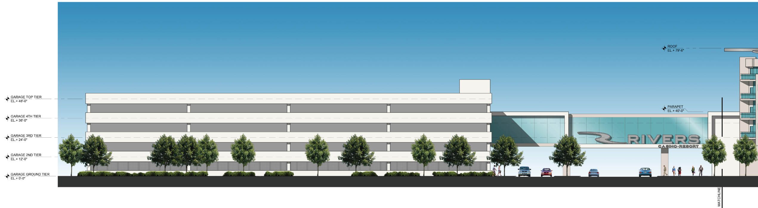
1 WEST OVERALL ELEVATION 1/16" = 1'-0"
