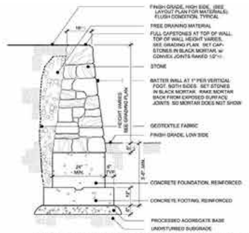
Stone Wall w/ Concrete Foundation Not to Scale
