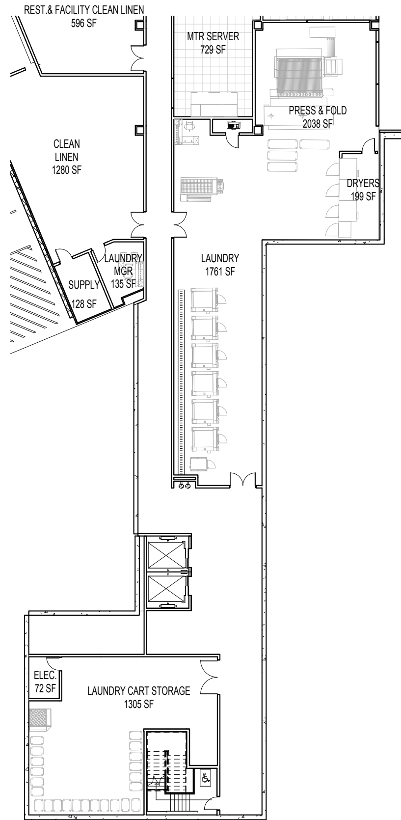
1 BOH - LL1 - LAUNDRY 3/64" = 1'-0"
