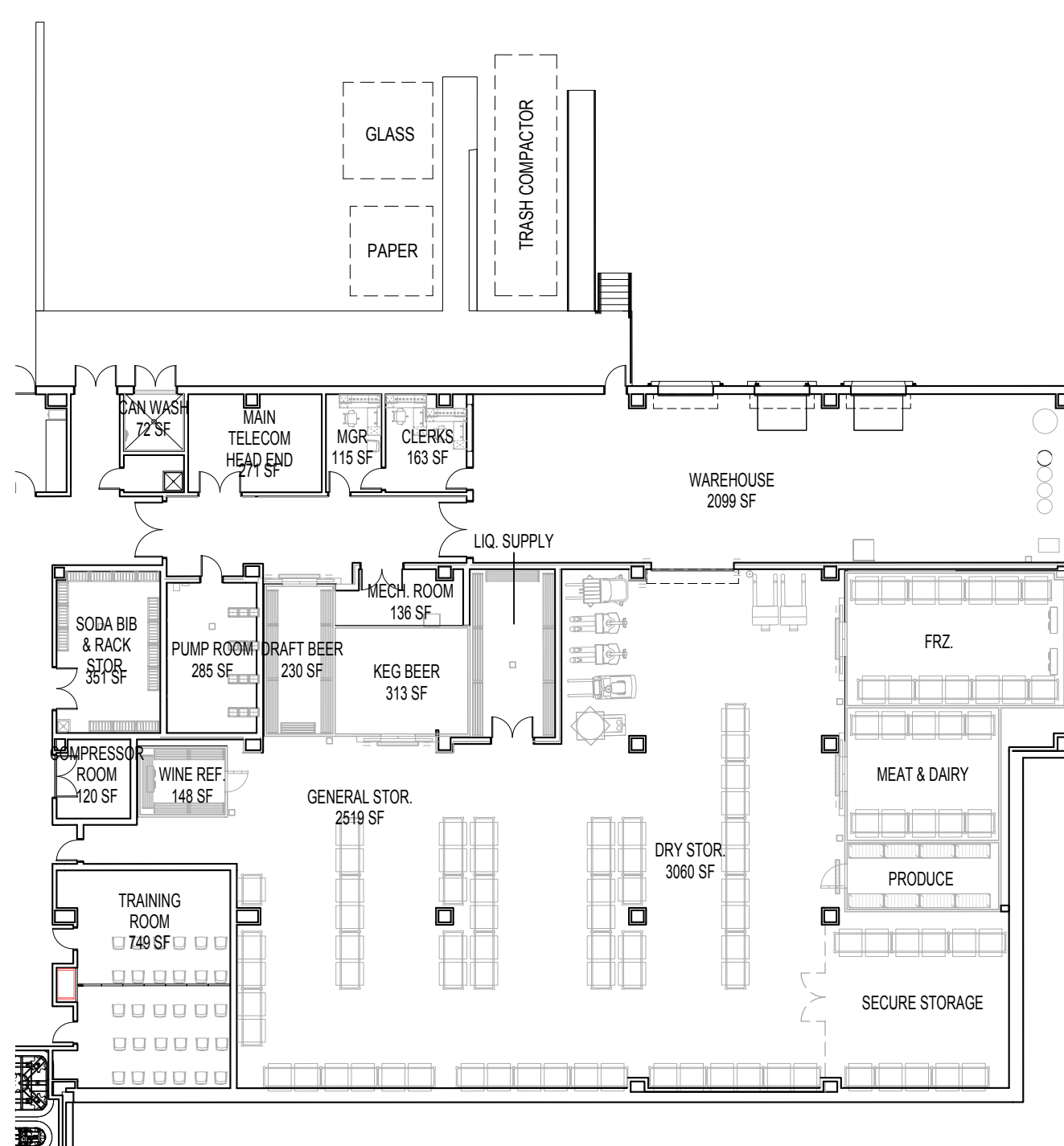
1 BOH - LL3 - WAREHOUSE 3/64" = 1'-0"
