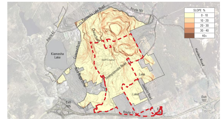
SLOPE ANALYSIS
