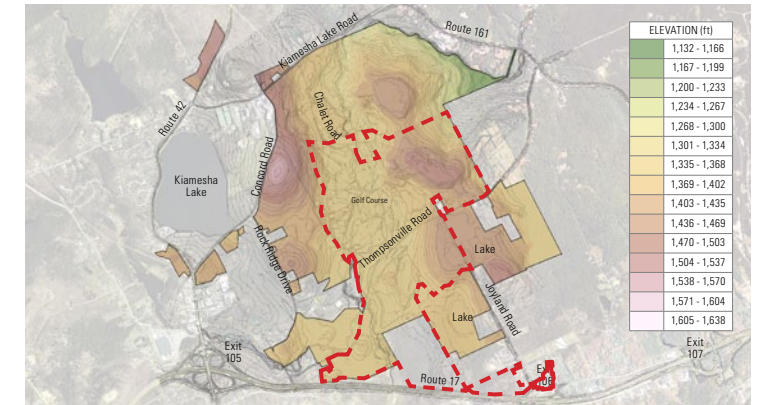
ELEVATION STUDY
